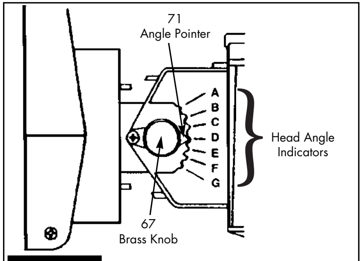
FIGURE 5 HEAD ANGLE INDICATORS
