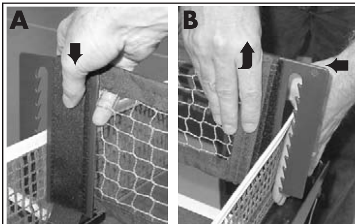
FIGURE 17 ATTACHING AND DETACHING THE SIDE NET (2050 ONLY)
