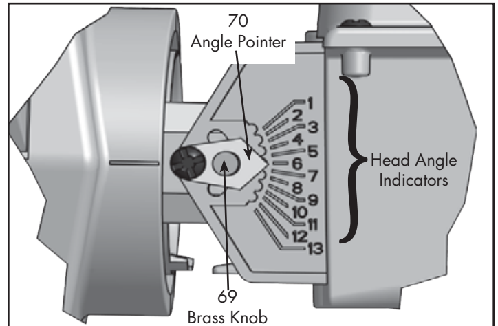
FIGURE 4 HEAD ANGLE INDICATORS
