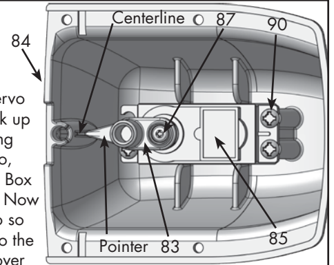
FIGURE B OSC. DRIVE PIN ALIGNMENT
